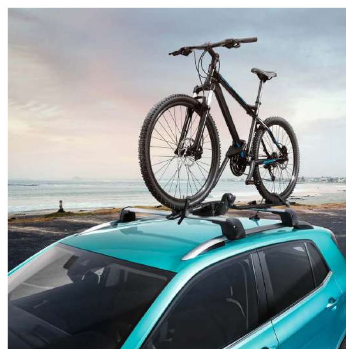
Bicycle holder For bicycle frames of up to 100 mm (oval)/80 mm (round)
